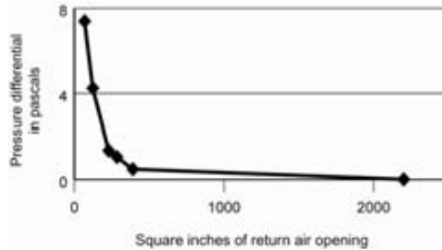
Figure 3-12 Master bedroom-living area pressure differential in the double section home
