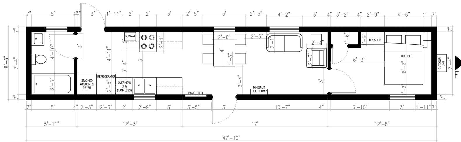
EXPRESS UNIT (NON-UFAS) – SCHEMATIC LAYOUT
