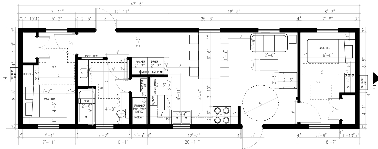
2-BEDROOM (ENHANCED) – SCHEMATIC LAYOUT
