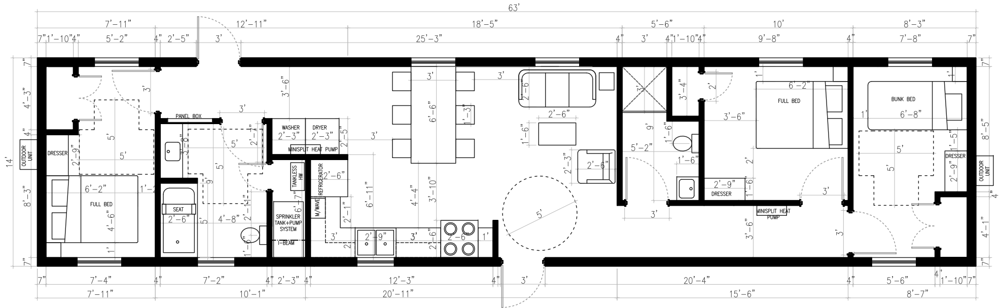
3-BEDROOM (ENHANCED) – SCHEMATIC LAYOUT
