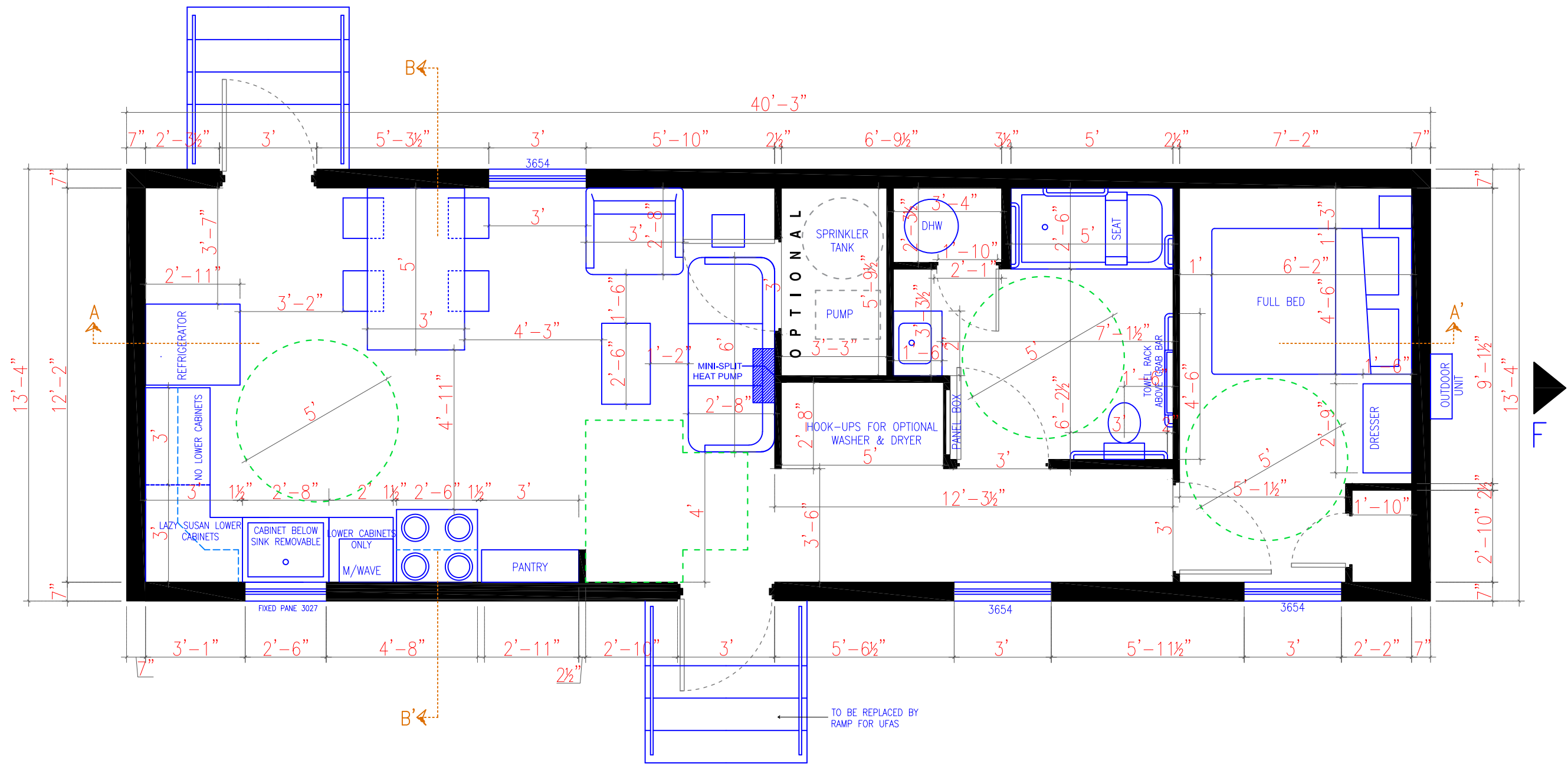
1 BEDROOM UNIT (UFAS) – PLAN WFA = 10.4%
