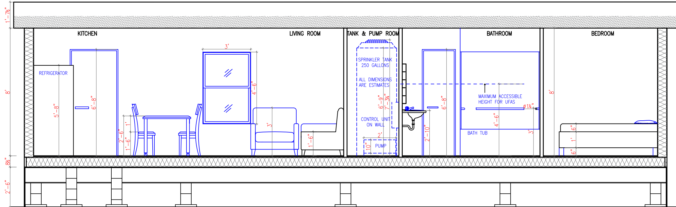
1 BEDROOM UNIT – SECTION AA' (6/24/2016)
