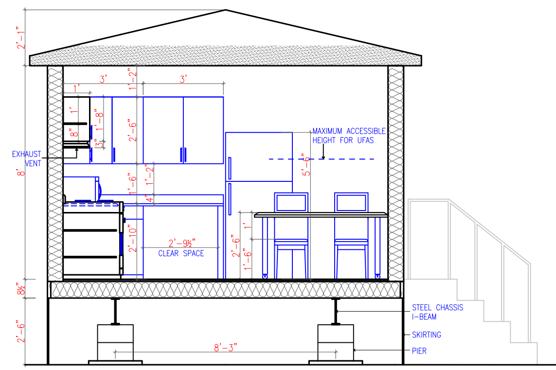
1 BEDROOM UNIT – SECTION BB' (6/24/2016)
