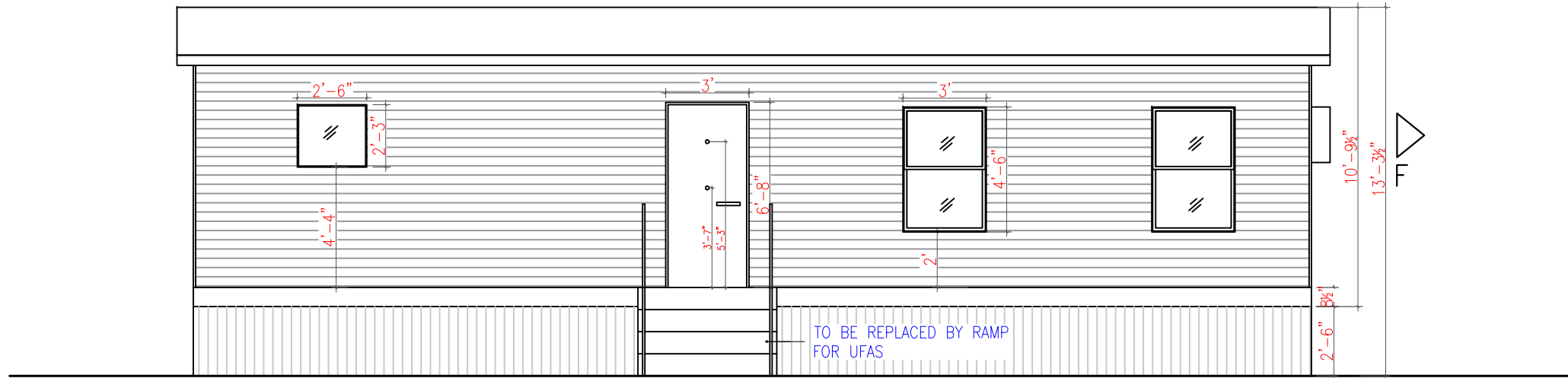
1 BEDROOM UNIT – RIGHT ELEVATION (6/24/2016)
