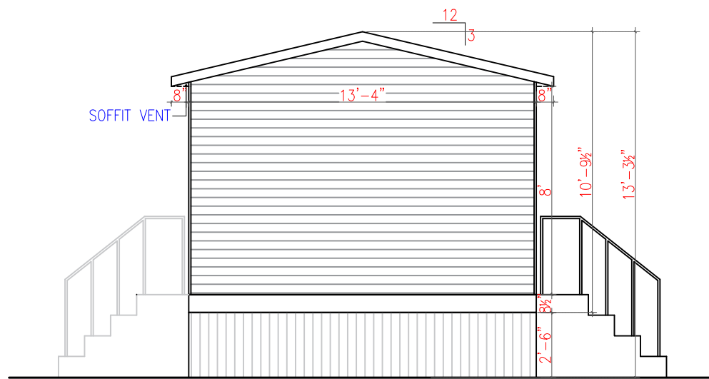
1 BEDROOM UNIT – REAR ELEVATION (6/24/2016)
