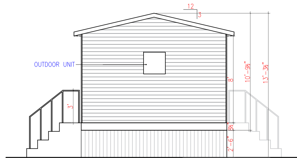
1 BEDROOM UNIT – FRONT ELEVATION (6/24/2016)
