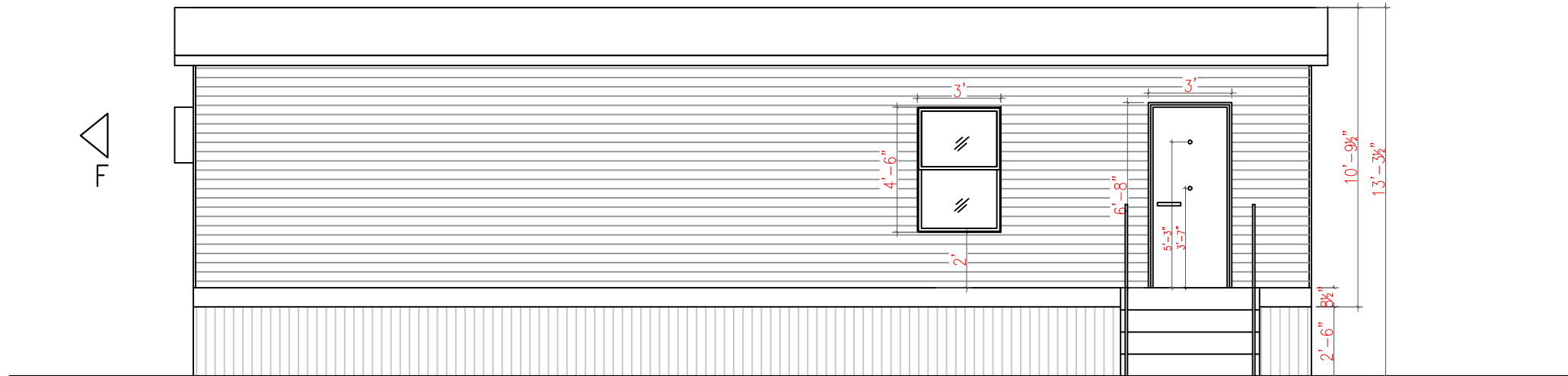
1 BEDROOM UNIT – LEFT ELEVATION (6/24/2016)
