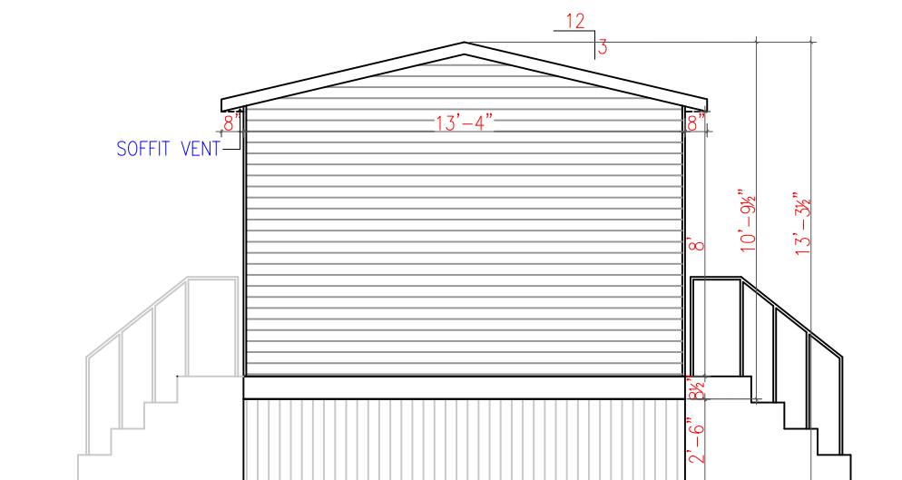
2 BEDROOM UNIT – REAR ELEVATION (6/24/2016)
