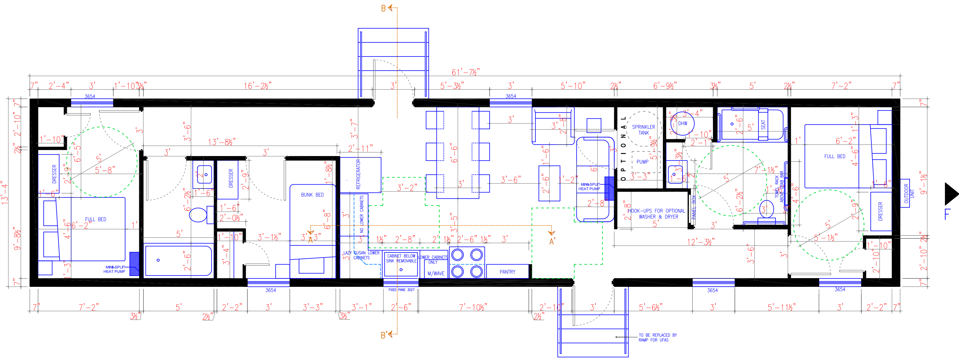
3 BEDROOM UNIT (UFAS) – PLAN WFA = 10.5% (6/24/2016)
