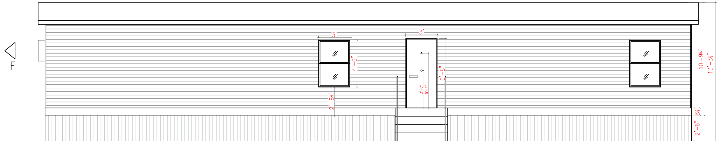
3 BEDROOM UNIT – LEFT ELEVATION (6/24/2016)
