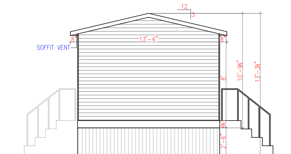
3 BEDROOM UNIT – REAR ELEVATION (6/24/2016)
