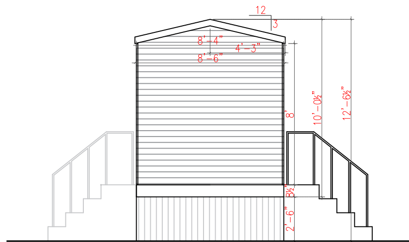
EXPRESS UNIT – REAR ELEVATION (6/24/2016)
