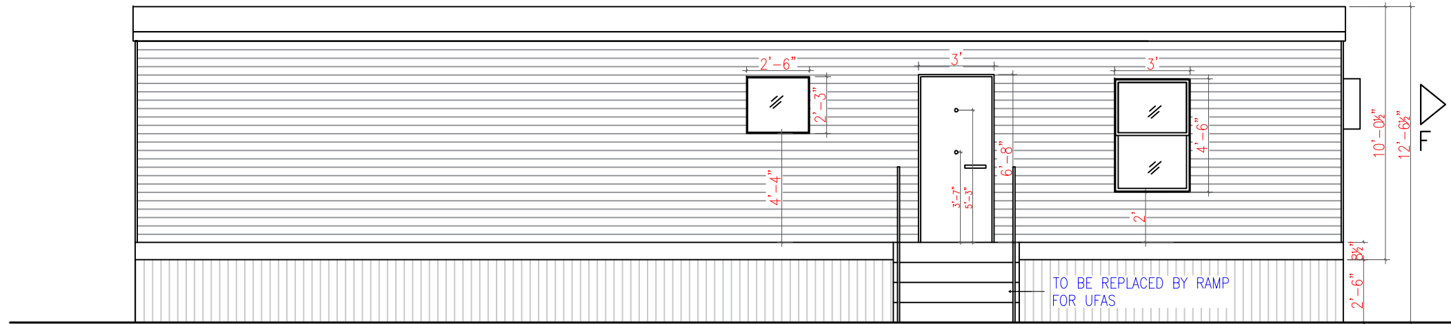
EXPRESS UNIT – RIGHT ELEVATION (6/24/2016)
