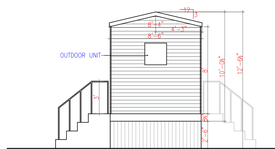
EXPRESS UNIT – FRONT ELEVATION (6/24/2016)
