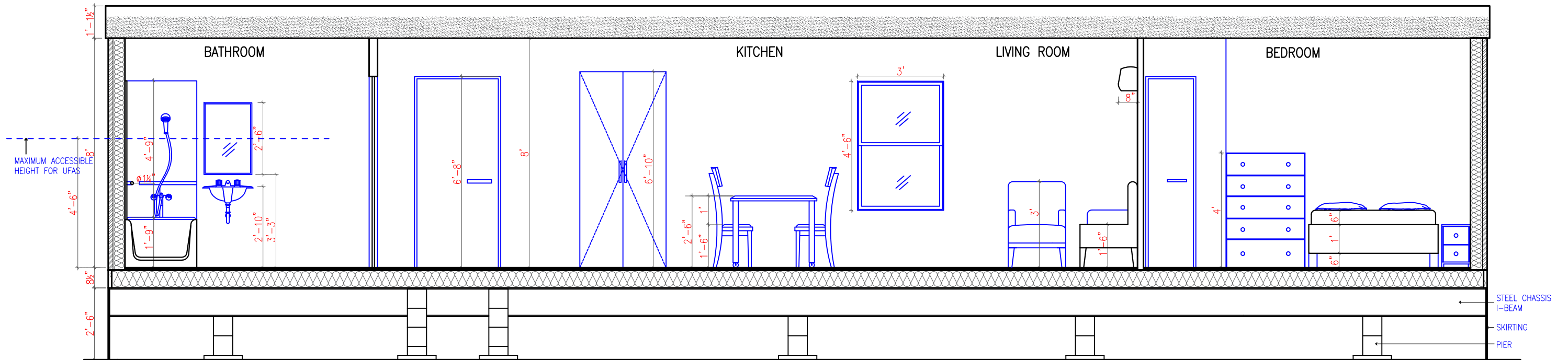
EXPRESS UNIT – SECTION BB' (6/24/2016)
