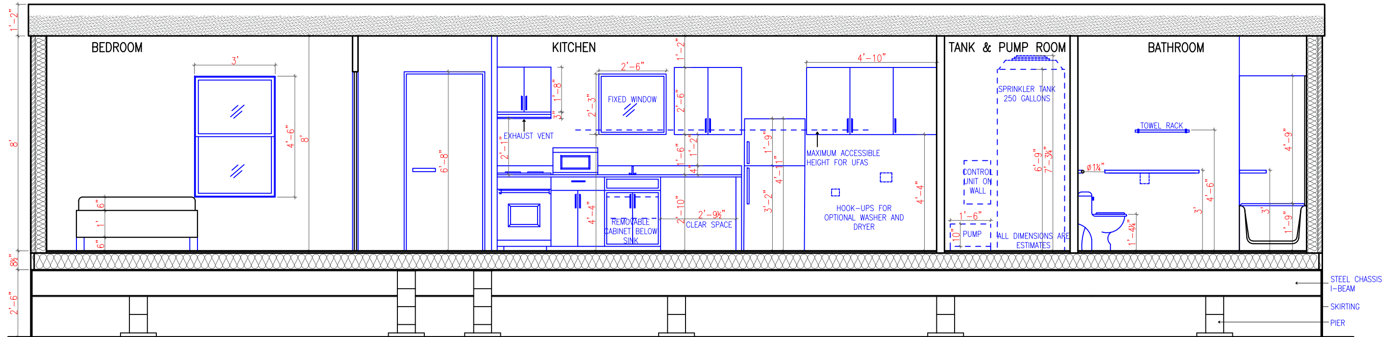
EXPRESS UNIT – SECTION AA' (6/24/2016)
