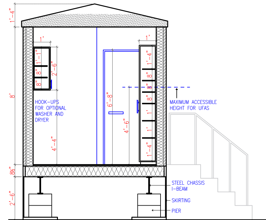
EXPRESS UNIT – SECTION DD' (6/24/2016)
