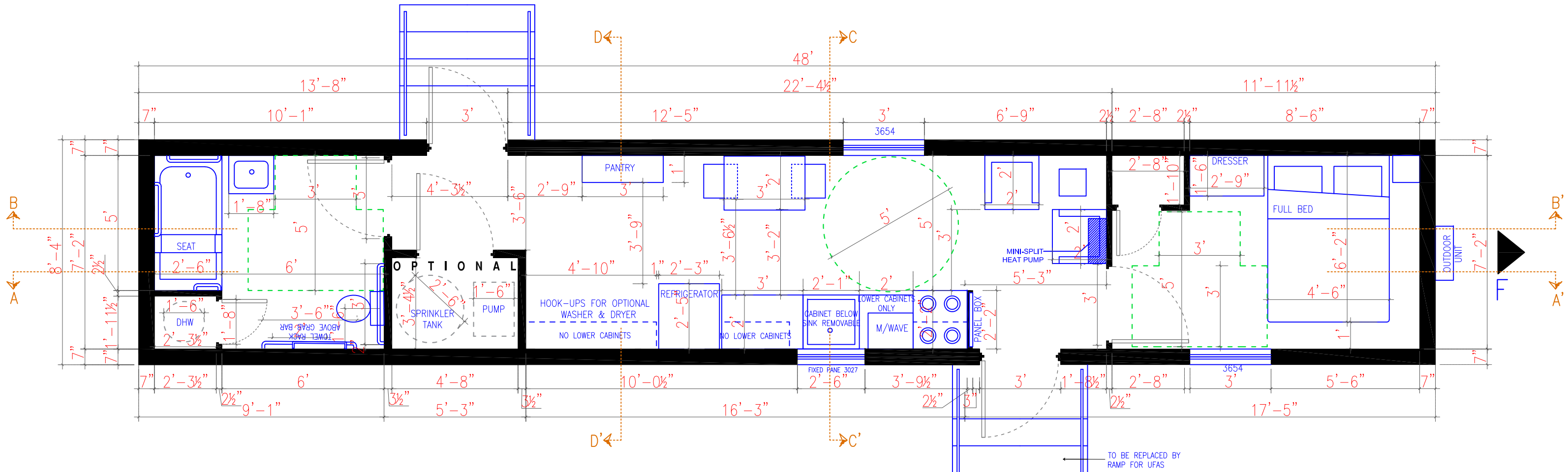
EXPRESS UNIT (UFAS) – PLAN WFA = 10.5% (6/24/2016)
