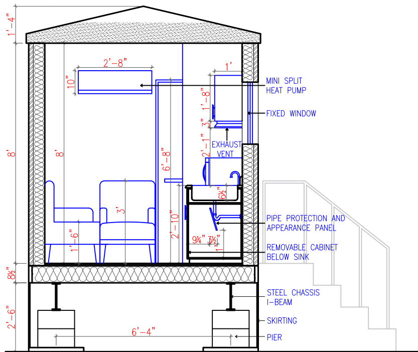
EXPRESS UNIT – SECTION CC' (6/24/2016)
